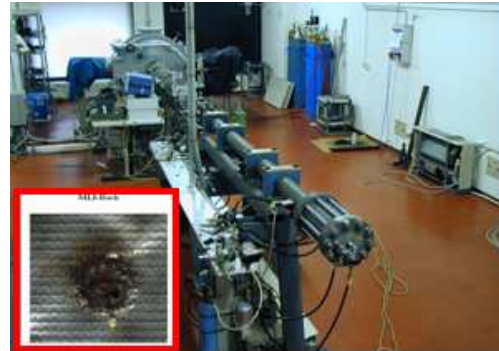
Fig. 2. FLECS impact testing
